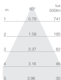
LED GU10 5W 60°
